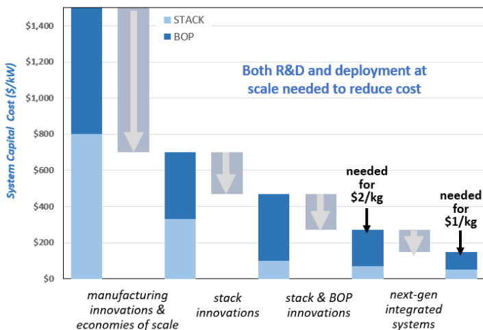
Figure 20: Reducing electrolyzer capital costs will require reaching economies of scale and innovating the electrolyzer stack and balance-of-plant components
